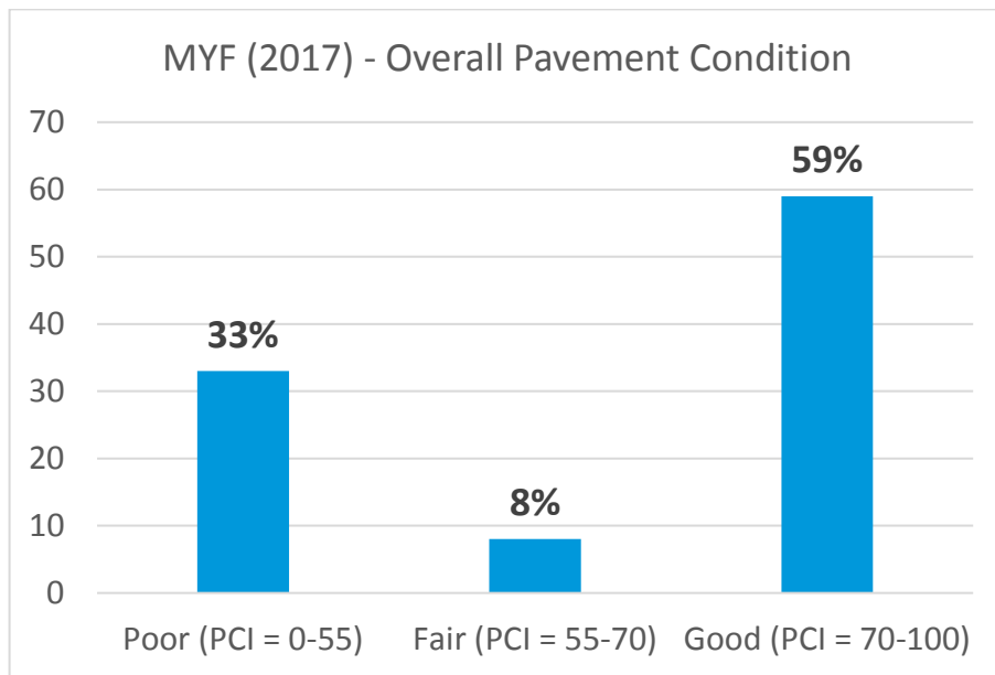
Figure 3-2 Overall Pavement Condition (August 2017)
